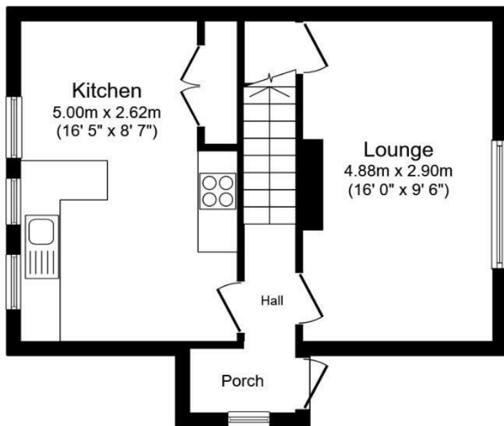
Ground Floor Floor area 36.8 sq.m. (396 sq.ft.)
